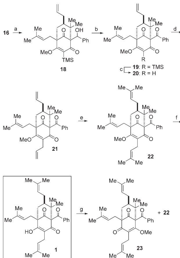
Scheme 5. Synthesis of nemorosone ( 1 ). Reagents and conditions: a) i\text{PrMgCl} , -78^{\circ}\text{C} , THF then \text{PhCHO} , -78 to 0^{\circ}\text{C} ; b) Dess–Martin periodinane, \text{CH}_2\text{Cl}_2 , RT; c) TBAF, THF, RT, 61 % (3 steps); d) LDA, THF, -78^{\circ}\text{C} , then lithium 2-thienylcyanocuprate, then allyl bromide, 88 %; e) Grubbs' 2nd generation cat., 2-methylpropene, 40^{\circ}\text{C} , 91 %; f) \text{LiI} , 2,4,6-collidine, 140^{\circ}\text{C} , 31 %; g) diazomethane, ether, 0^{\circ}\text{C} , 60 % for 23 and 7 % for 22 . TBAF = tetrabutylammonium fluoride.
